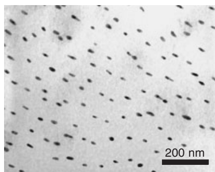
Figure 2. TEM image of an ensemble of touching core-shell colloids after 30 MeV Se ion irradiation at a fluence of 2 \times 10^{14} \text{ cm}^{-2} . Aligned Au nanorods with varying size aspect ratios are observed.
