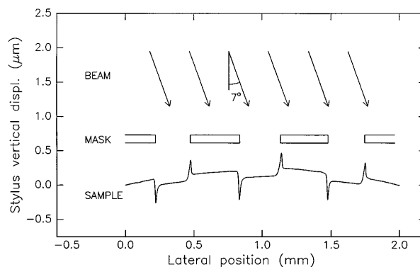
FIG. 1. Surface profile of a c -InP substrate implanted through a contact mask with 30 MeV, 10^{15} Se/cm 2 at 7° off normal.
