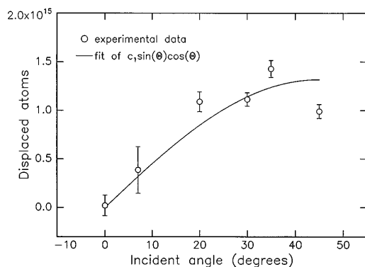
FIG. 4. Number of displaced atoms along 1 cm as a function of angle \theta between ion beam and surface normal. Samples were implanted with 24 MeV, 3 \times 10^{14} Se/cm 2 .
