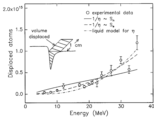
FIG. 3. Number of atoms along 1 cm, displaced by 3 \times 10^{14} Se/cm 2 as a function of initial ion energy. Also shown are the estimates of the total mass transport using a viscosity inversely proportional to S_n (solid line), S_e (dashed line), and with a liquidlike behavior viscosity (dashed-dotted line).
